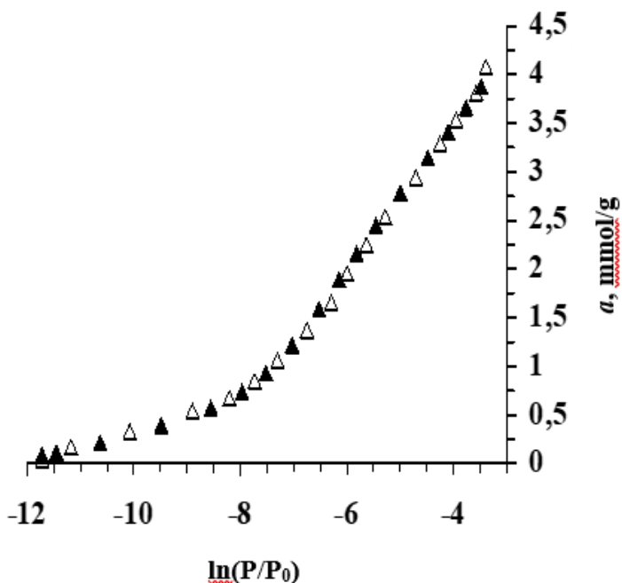
Fig. 1. Hydrogen sulfide adsorption isotherm in LiX zeolite at 303 K. \Delta -experimental value; \blacktriangle -value of the point, calculated on the basis of the equations of the theory of volumetric filling of micropores.
