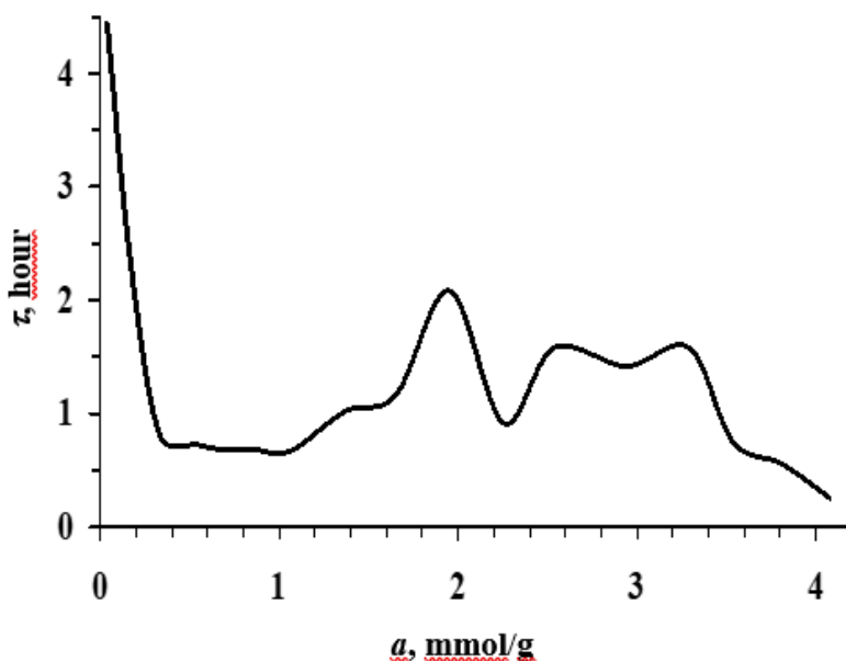
Fig. 4. The set-time of the adsorption equilibrium, depending on the size of the adsorption of benzene in the zeolite LiX at 303K.
