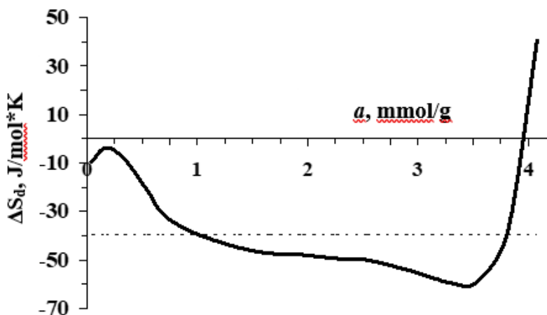
Fig. 3. The differential entropy of the сероводород adsorption in the zeolite LiX at 303K. Entropy of liquid сероводород is taken as zero. The horizontal dashed line – mean molar integral entropy.
