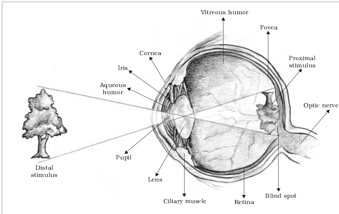
Fig.5.1 : Structure of the Human Eye
