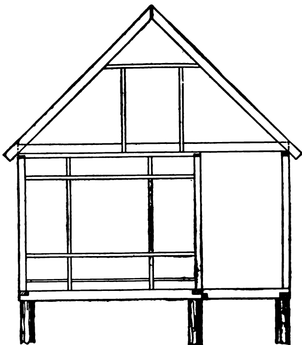
FIG. 396. END ELEVATION.
