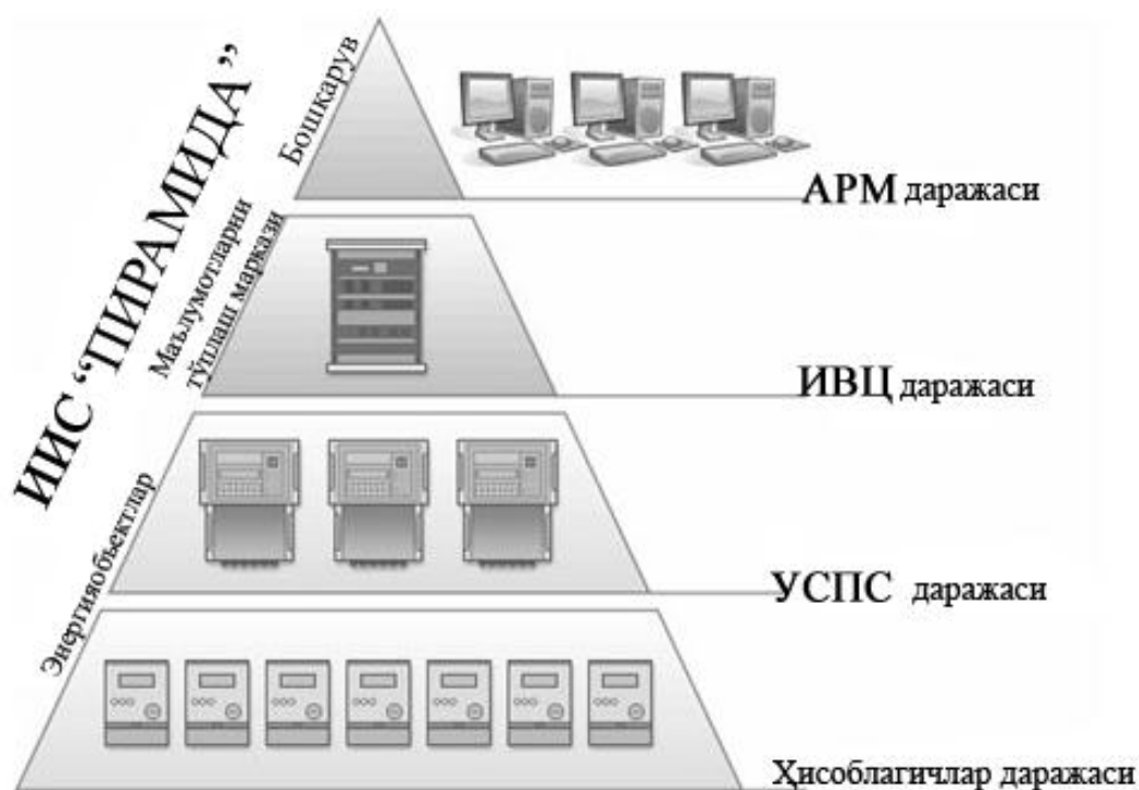
1-rasm. IIS "Piramida" sxemasi
