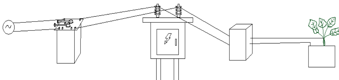
Fig. 4. Process of electric pulse treatment of tomato and cucumber roots not removed from the soil
