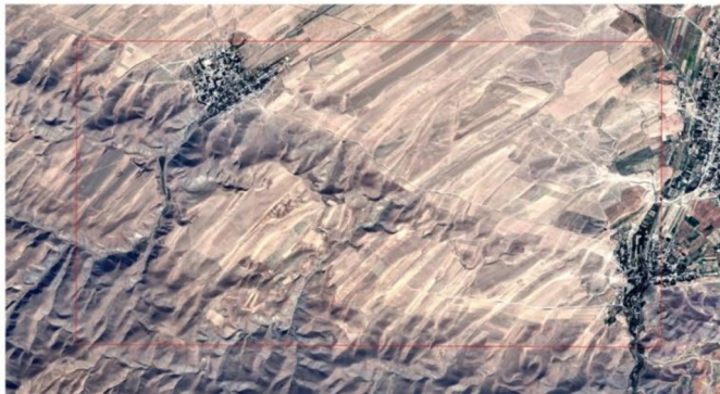
Fig. 2. Processed satellite image Landsat 7 on territory of Ardakshan prospective area (Materials of SE "IMR"). Scale 1:25000
