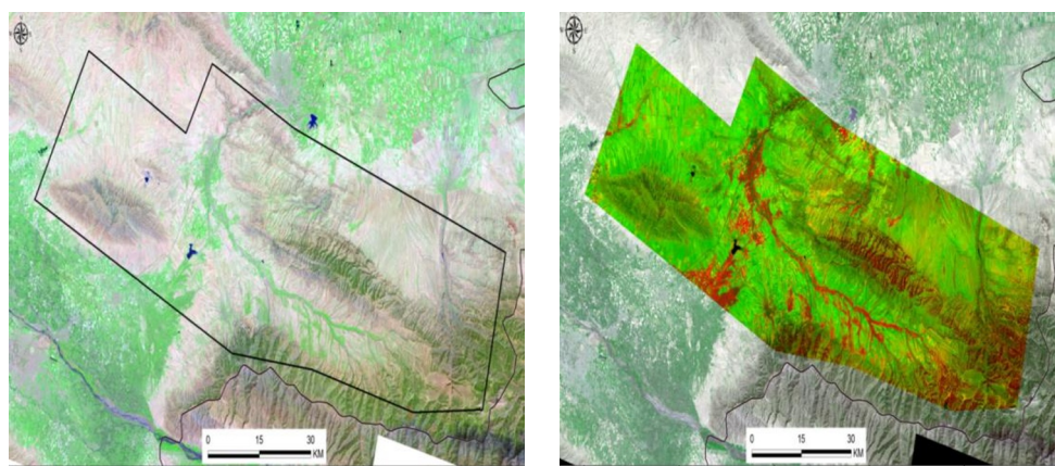
Fig 1. Processed satellite image Landsat 7
