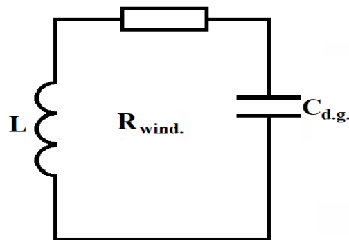
Figure 5. Equivalent circuit of the high-voltage circuit of the ozone generator: L - inductance of the secondary winding of the step-up transformer; C_{d.g.} - capacity of the discharge gap; R_{wind.} - active resistance of the secondary winding of the transformer
