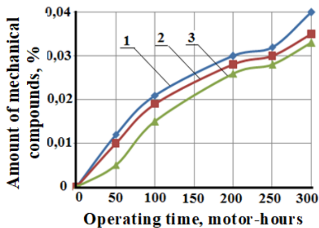
Figure 1. When using Agrimot SDX 15w-40 motor oil in the engine "in different climatic conditions", the dynamics of changes in its composition of mechanical mixtures. 1 - Surkhandarya region;2 - Fergana region;3 – Tashkent region
