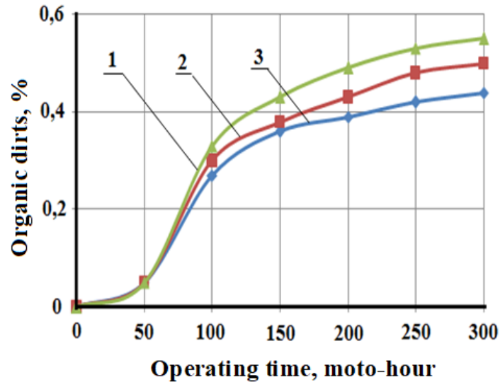
Figure 2. Dynamics of change of organic impurities in oil. 1 - Surkhandarya region; 2 - Fergana region; 3 – Tashkent region
