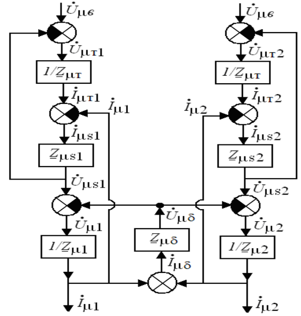
Fig.2. PSD of the magnetic circuit of electromagnetic transducers
