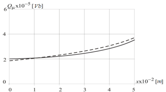
Fig. 4. The curves of change of the magnetic flux along the magnetic circuit: solid line - estimated; the dotted line – pilot As shown from results of research of the influence of non-linearity of the magnetization curve for the primary flow distribution in a magnetic circuit electromagnetic transducer of three-phases current ranges identified characteristic changes in the magnetic induction. As a result of research for each band
