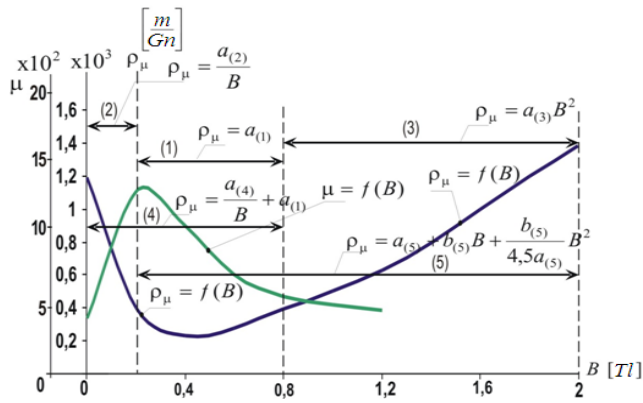
Fig. 3. Curves and specific magnetic resistance of the magnetic permeability of steel from induction
