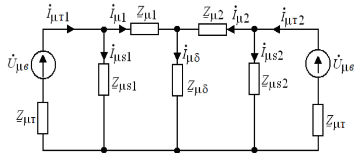
Fig. 1. The equivalent circuit of the magnetic circuit of the electromagnetic transducers of three-phase current
