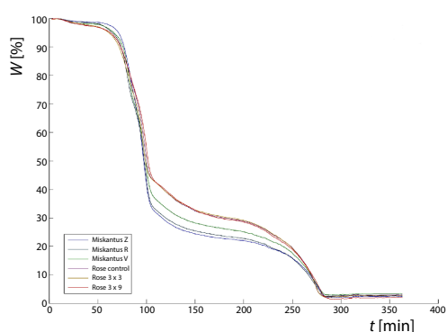
Figure 4. Changes in mass of analysed samples (for color image see journal web site)
