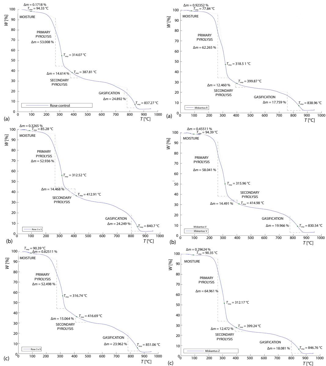
Figure 2. The TGA curves for RM ; (a) control, (b) laser irradiated 3 × 3 seconds, and (c) 3 × 9 seconds
