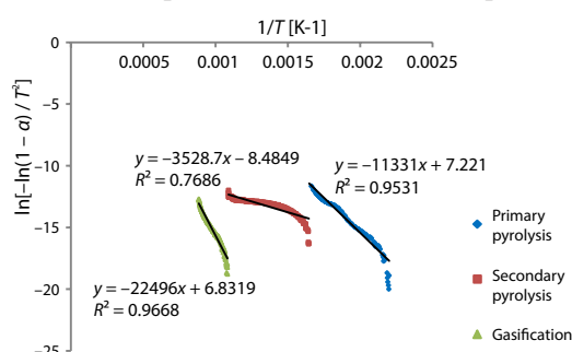
Figure 5. The slope of a plot \ln[-\ln(1 - \alpha)]/T^2 against 1/T (for color image see journal web site)
