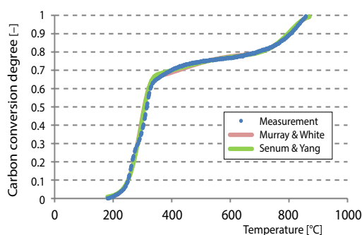
Figure 6. Fit of models to the experimental data (for color image see journal web site)
