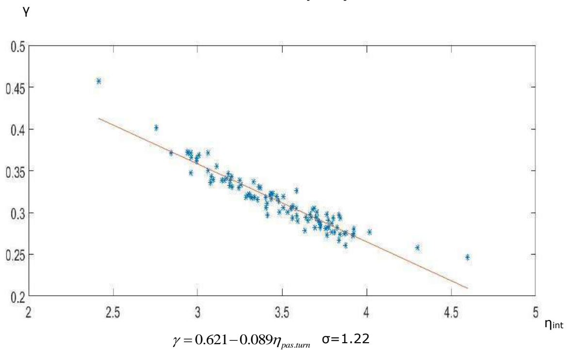
Figure 2. Graph of dependence of the coefficient of passenger interchange the coefficient of capacity utilization
