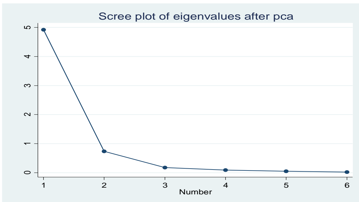
Figure 1. Scree plot of eigenvalues of PCA analysis on 6 WGI indexes of institutional quality.
