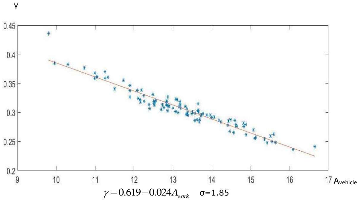
Figure 1. Graph of the correlation of the number of buses on the route coefficient of capacity utilization
