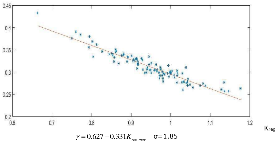
Figure 3. Graph of dependence of the coefficient of regularity on the coefficient of capacity utilization
