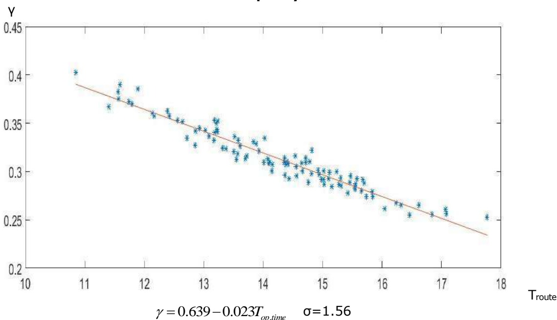
Figure 4. Graph of the dependence of the time of stay of the bus in the direction on the coefficient of capacity utilization
