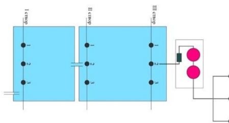
Fig. 2. Sampling scheme of turbidity in the clarifier of drip irrigation system of "Korateri Botir cotton" farm.
