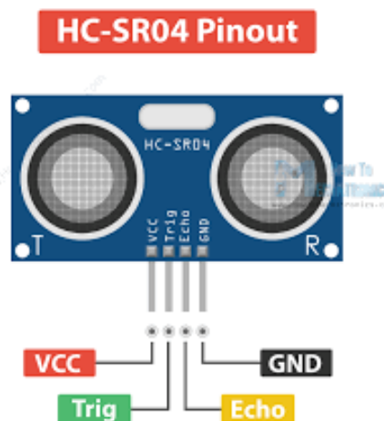
Figure 3. Pin configuration of the ultrasonic sensor (HC-SR04)
