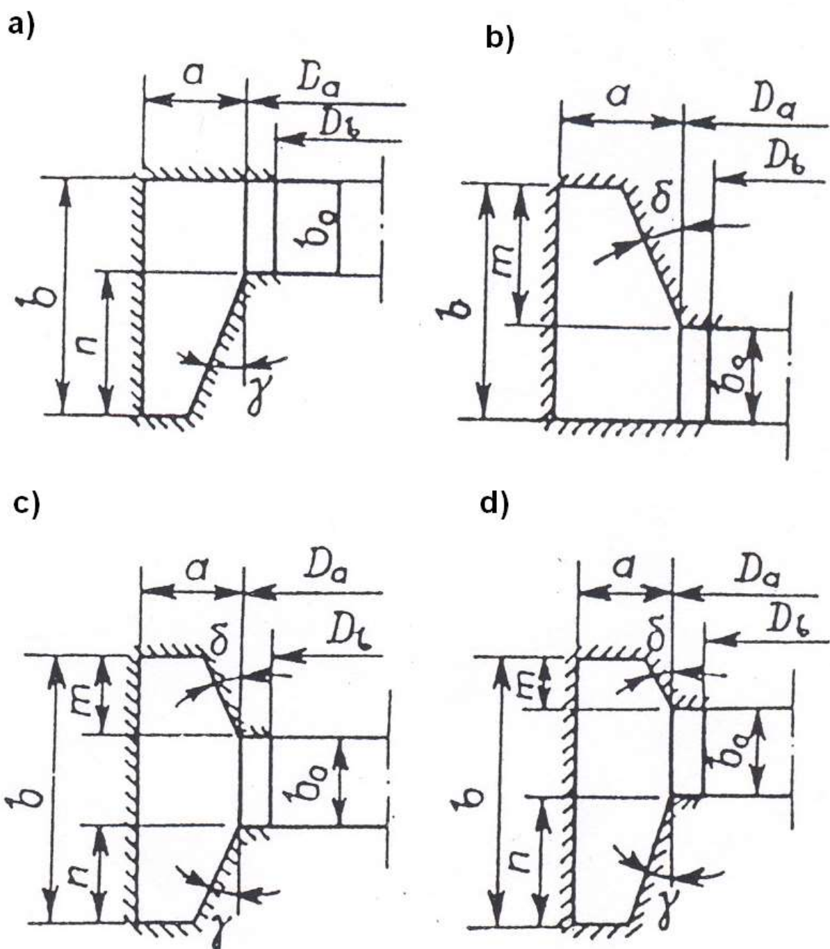
Rasm 2.10. Beton spiral kameralar qirqim formalari
