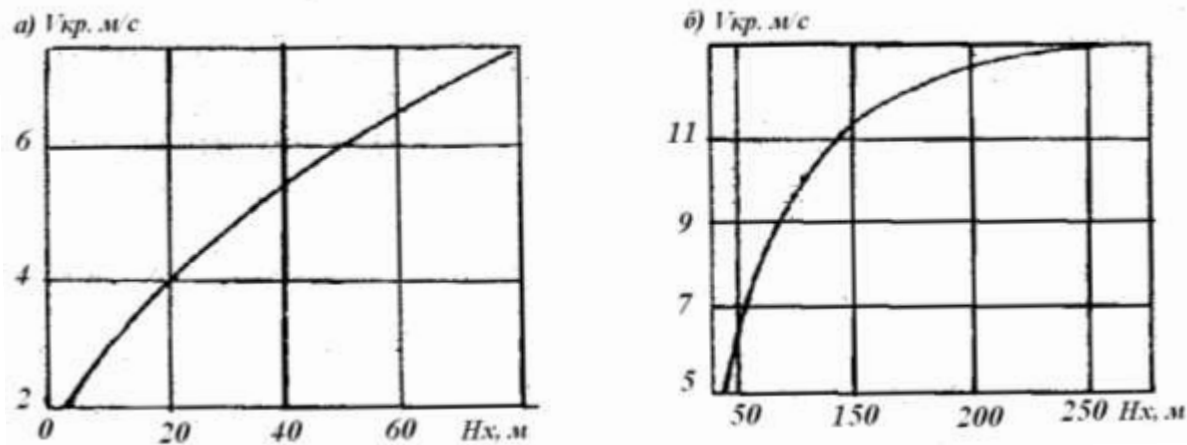
12-rasm. Naporga qarab spiral kameraga V_{kr} - kirish tezligini aniqlash: a- betonli; b- metali spiral kamera; \phi_{kr} – kirish kesimining tezlik koeffitsienti
