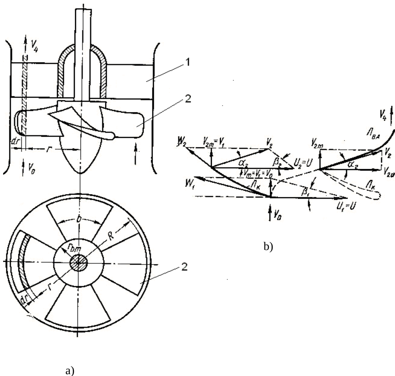
Rasm 1.36. Ukiy nasos (a) va undagi okimning kinematikasi (b). 1 – tugrilovchi apparatning parraklari; 2 – ish gildiragi parraklari
