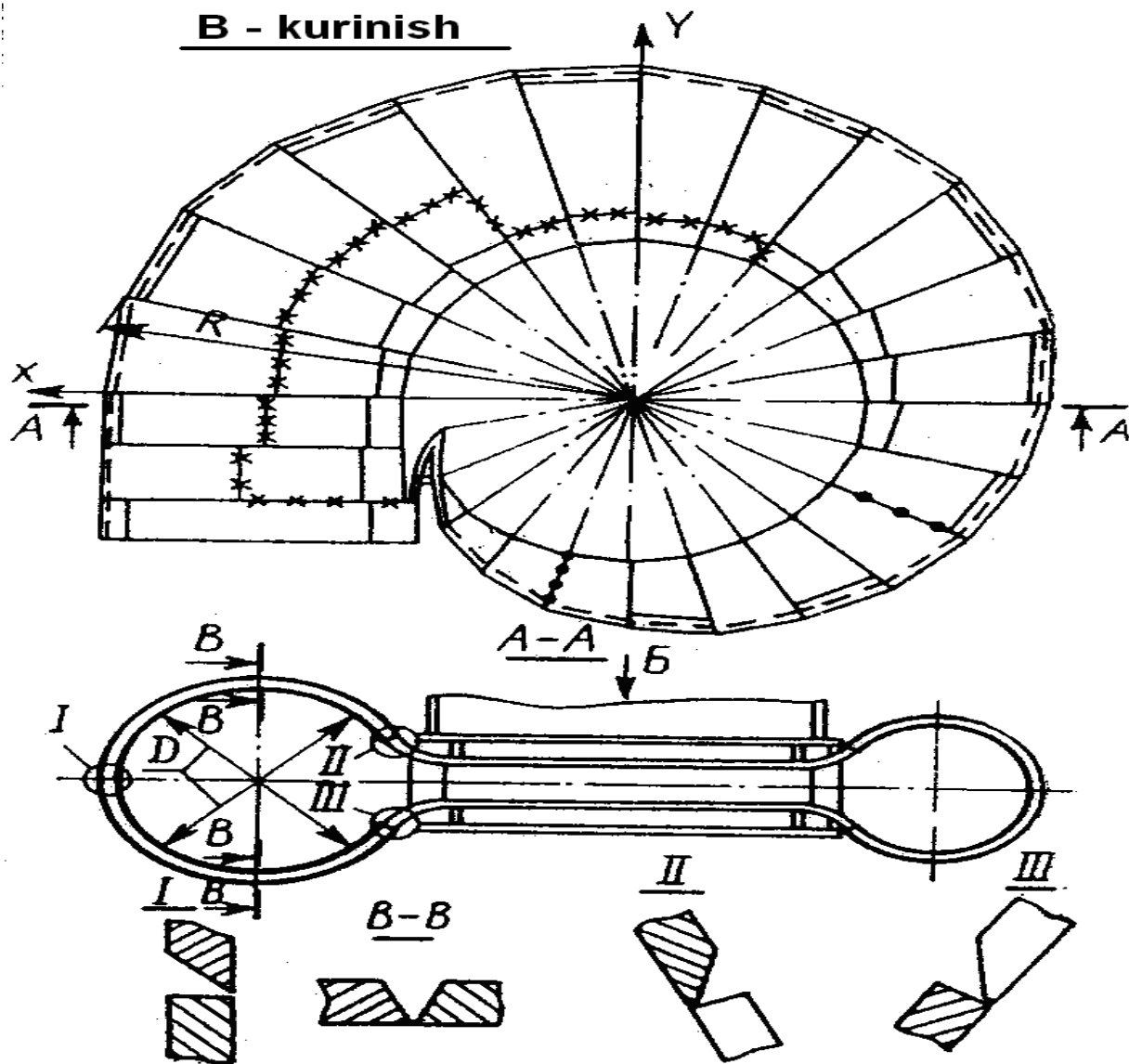
Rasm 2.14. Metal spiral kamera materiallari markasiga qarab taqsimlanishi prinsipial sxemasi
